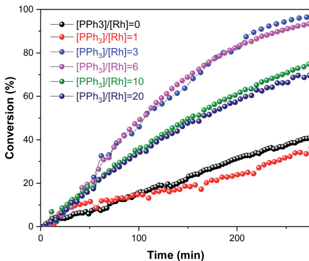
Fig. 6 Substrate conversion profiles of [\text{Rh}(\text{CO})_2(\text{acac})] + \text{PPh}_3 catalysed hydroformylation of 1-hexene in toluene at 50\text{ }^\circ\text{C} and 12 bar of \text{H}_2/\text{CO} (1 : 1) monitored using operando ^1\text{H} FlowNMR spectroscopy. [\text{Rh}(\text{CO})_2(\text{acac})] = 2.5\text{ mM} , [\text{1-hexene}] = 500\text{ mM} , [\text{PPh}_3] varied as indicated.
