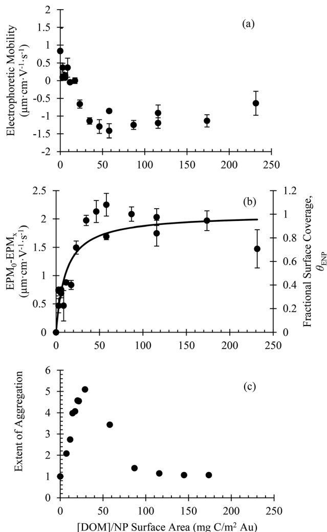
Fig. 2 (a) Electrophoretic mobility of bPEI-AuNPs (5 mg L -1 ); (b) change in electrophoretic mobility and fractional surface coverage ( \theta_{ENP} ) of bPEI-AuNPs (5 mg L -1 ); and (c) extent of homoaggregation of bPEI-AuNPs (2 mg L -1 ) in the presence of SRNOM. Error bars represent one standard deviation of replicates. Solution conditions included 1 mM HEPES, 20 mM NaCl and varying SRNOM concentrations.
