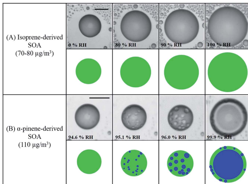
Fig. 35 Optical images of micrometer scale SOA particles with increasing relative humidity. (a) Isoprene-derived SOA for mass concentrations of 70–80 \mu\text{g}\text{m}^{-3} and (b) \alpha -pinene-derived SOA for a mass concentration of 110 \mu\text{g}\text{m}^{-3} . Note that the light gray circles at the center of the particles are due to an optical effect caused by the hemispherical shape of the particles deposited on a substrate. Illustrations are shown below the images for clarity. Green: organic-rich phase. Blue: water-rich phase. The scale bar represents 20 \mu\text{m} . Reproduced from ref. 327 under Create Commons License (CC BY-NC-ND 4.0) from the American Geophysical Union, © The Authors, 2017.
