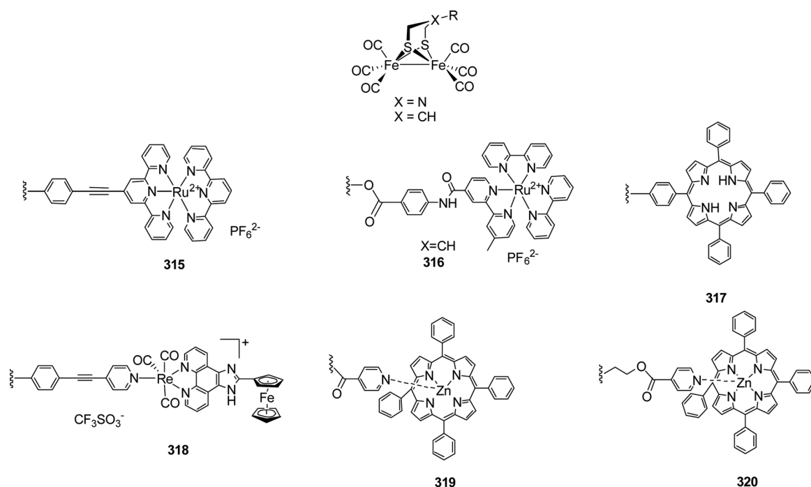
Fig. 109 Models 315 to 320. Examples of \text{Fe}_2(\text{xd}^{\text{R}})(\text{CO})_6 models modified for photocatalytic purposes.
