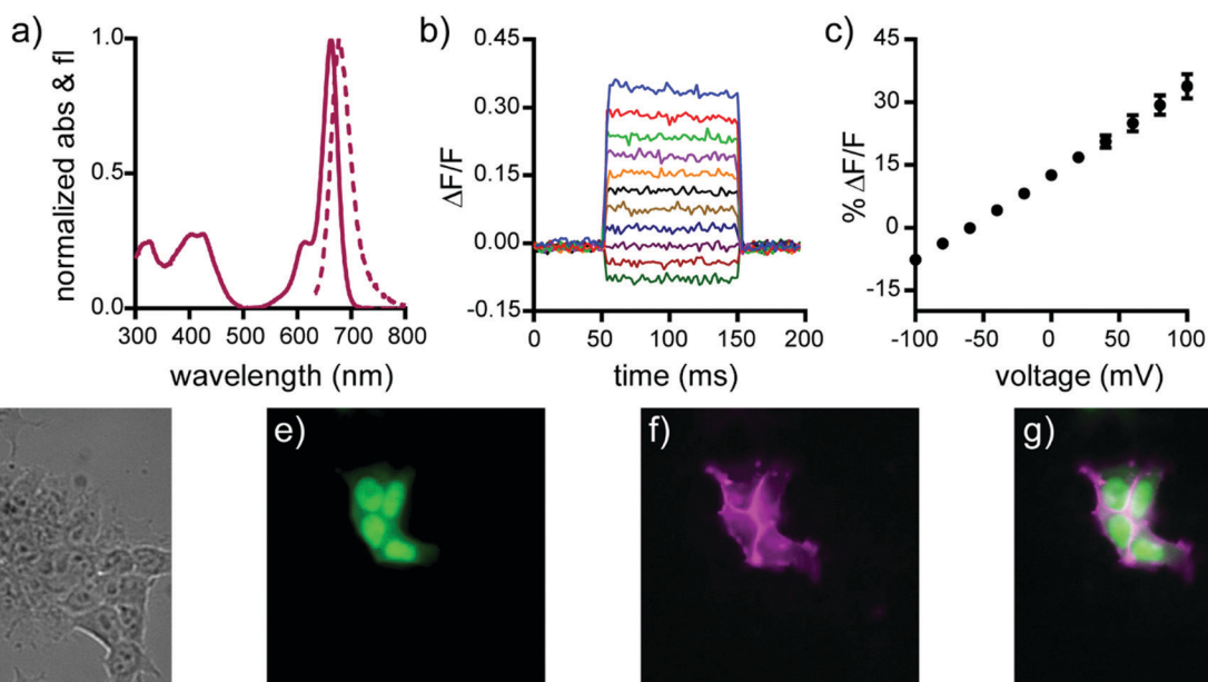
Fig. 1 Cellular and in vitro characterization of isoBeRST-Halo 7. (a) Normalized absorbance (solid line) and emission (dashed line) spectra of isoBeRST-Halo 7 in PBS, pH 7.4. (b) Plot of the fractional change in fluorescence of 7 vs. time for 100 ms hyper- and depolarizing steps ( \pm 100 mV in 20 mV increments) from a holding potential of -60 mV for single HEK cells under whole-cell voltage-clamp mode. (c) Plot of \% \Delta F/F vs. final membrane potential. Data are mean \pm S.D. for n = 6 cells. (d–g) Wide-field microscopy images of HEK cells transfected with CMV-HaloTag-pDisplay and stained with isoBeRST-Halo 7 (50 nM, 30 min). (d) DIC image of HEK cells. (e) Nuclear EGFP fluorescence indicates HaloTag expression. (f) isoBeRST-Halo fluorescence. (g) Merge of fluorescence from EGFP (green) and isoBeRST-Halo (magenta). Scale bar is 10 \mu\text{m} .
