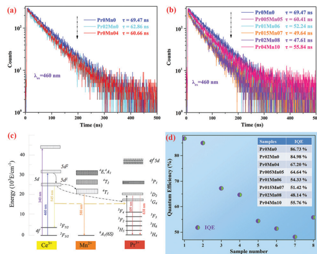
Fig. 8 Fluorescence decay curves: (a) Pr0Mn0, Pr0Mn04. (b) Pr0Mn0, Pr005Mn05, Pr01Mn06, Pr015Mn07, Pr02Mn08, Pr04Mn10. (c) Schematic of the energy transfer process among \text{Ce}^{3+}\text{-Pr}^{3+}\text{-Mn}^{2+} ions. (d) Internal quantum efficiencies (IQEs) of the TCs under 460 nm excitation.
