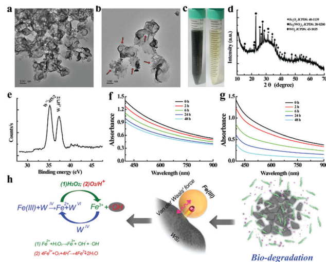
Fig. 5 (a and b) Morphology of \text{Fe(III)}@ \text{WS}_2 -PVP nanocapsules (observed using TEM) after being stored in PBS for 72 h (scale bar = 100 nm); (f) time-dependent light absorbance of \text{Fe(III)}@ \text{WS}_2 -PVP nanocapsules in PBS; (c) solution images of \text{Fe(III)}@ \text{WS}_2 -PVP nanocapsules after being stored in PBS for 0 day (fresh solution: left) and 7 days (right); (g) time-dependent light absorbance of \text{Fe(III)}@ \text{WS}_2 -PVP in buffer solution with lower pH; (d) XRD and (e) XPS of 7 day-degradation products in PBS; and (h) enhanced biodegradation and DOX release mechanism of \text{Fe(III)}@ \text{WS}_2 -PVP nanocapsules. Yellow balls: \text{Fe(III)} species; pink balls: DOX; green lines: PVP. The left picture of panel (h) shows the repeated redox reaction and \text{H}_2\text{O}_2 and \text{H}^+ accelerated the biodegradation process of \text{Fe(III)}@ \text{WS}_2 -PVP nanocapsules. Reprinted from ref. 103. Copyright 2017 John Wiley & Sons.
