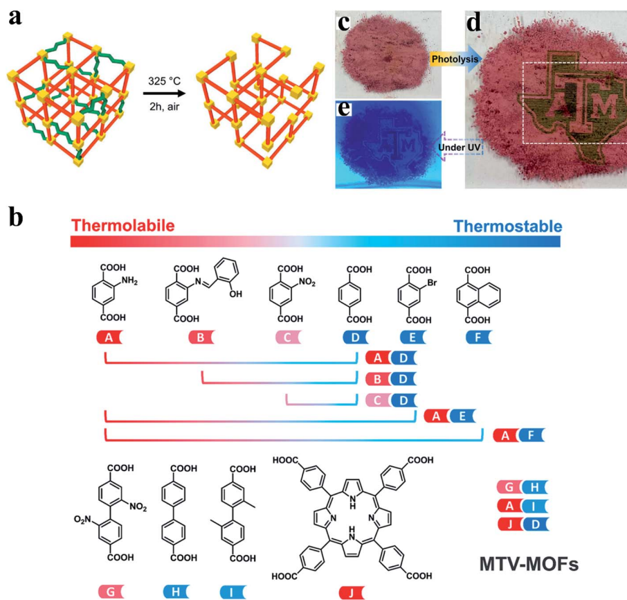
Fig. 4 (a) Defect creation by decomposing the labile linkers (green) in the stable (red) matrix. Yellow: Zr nodes. Reproduced with permission. 65 Copyright 2017, American Chemical Society. (b) The versatility of controllable linker thermolysis to construct HP-MOFs with various linkers. Reproduced with permission. 66 Copyright 2018, American Chemical Society. Optical photographs of (c) the original UiO-66-TCPP-5% powder, (d) a logo on the UiO-66-TCPP-5% powder after programmable photolithography and (e) the patterned MOF sample under a UV lamp. Adapted with permission. 68 Copyright 2020, Wiley-VCH.
