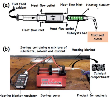
Fig. 36 (a) Schematic representation of the setup of a continuous flow system for the catalytic ODS and (b) the real experimental setup. Adapted from ref. 252b with permission from The American Chemical Society.
