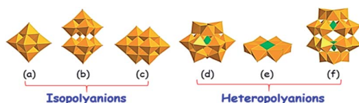
Fig. 15 Representation of the typical POM structure of (a) Lindqvist ([M 6 O 19 ] 7− ), (b) decatungstate ([W 10 O 32 ] 4− ), (c) decavanadate ([V 10 O 28 ] 6− ), (d) Keggin ([XM 12 O 40 ] n− ), (e) Anderson ([H x (M' 6 O 6 )M 6 O 18 ] n− ) and (f) Dawson ([X 2 M 18 O 62 ] n− ). Adapted from ref. 95 with permission from Elsevier.
