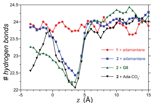
Fig. 5 Total number of hydrogen bonds between water and the four rim carboxylates of OA 1 and exo-OA 2 as a function of the position ( z ) of the guests adamantane, G8, and adamantane carboxylate (Ada-CO _2^- ) along the cavitand C_4 -axis of symmetry. The position ( z ) was defined by the zero-plane perpendicular to the C_4 -axis of symmetry – itself defined by the eight ether-oxygens atoms at the rim of the pocket – and the center of mass of the adamantane guest as it was moved along the C_4 host axis. Error bars have been neglected for clarity, however, the error in the number of hydrogen bonds at a given separation z is 0.25.
