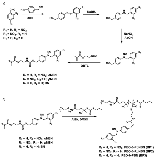
Scheme 2 Synthetic routes of (a) NO-releasing monomers, \alpha\text{NBN} , p\text{NBN} , and \text{BN} and (b) amphiphilic diblock copolymers (BP1–BP3) through RAFT polymerization.
