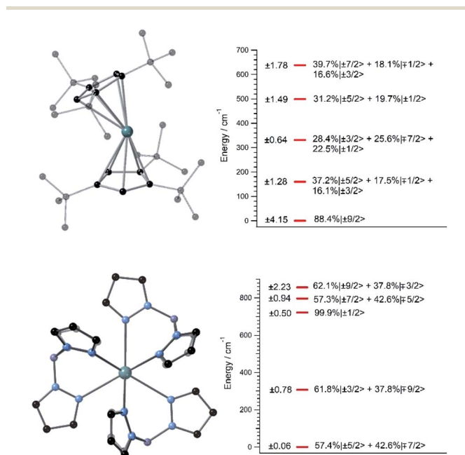
Fig. 1 (Left top and bottom) [U(Cp ttt ) 2 ] + and UTP 3 relaxed geometries. Hydrogen atoms are omitted for clarity. Green: U, black: C, blue: N, violet: B. (Right top and bottom) [U(Cp ttt ) 2 ] + and UTP 3 lowest 2J + 1 = 10 equilibrium energies with wave-functions on the right (amplitudes < 15% are not shown) and their J_z operator expectation values on the left. The wave-functions are written in terms of the ground J = 9/2 multiplet of U 3+ .
