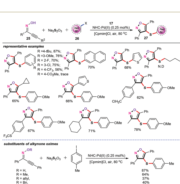
Scheme 12 Palladium-catalyzed cascade annulation/sulfenylation reaction.
