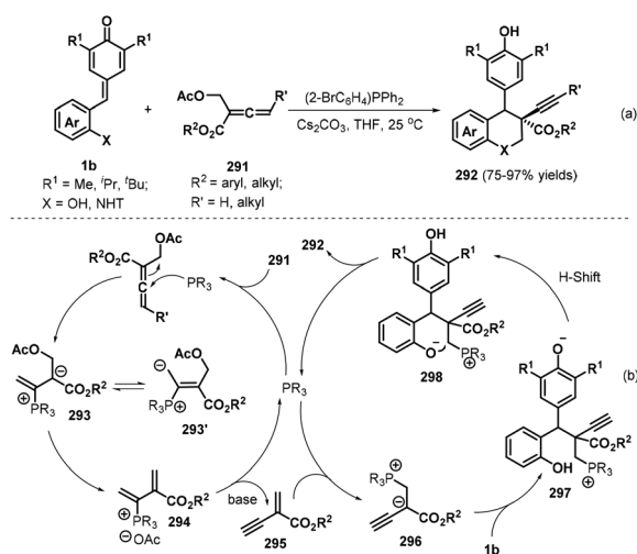
Scheme 64 [4 + 2] annulation of p -QMs with allenoates.
