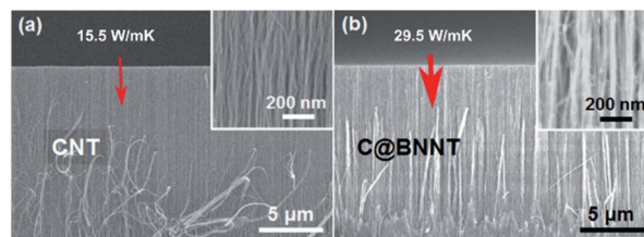
Fig. 13 Scanning electron microscopy (SEM) images of (a) VA-CNTs and (b) VA-MWCNTs coated in h-BN. The h-BN coating increased thermal conductivity of the aligned assembly from 15.5 W m -1 K -1 to 29.5 W m -1 K -1 . Reproduced with permission from ref. 22. Copyright 2017, American Chemical Society.
