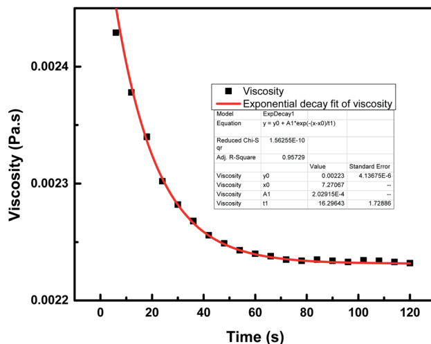
Fig. 10 Viscosity variation of 7-PSC in 15W-40 engine oil (base fluid) with time at a constant shear rate of 100 \text{ s}^{-1} .
