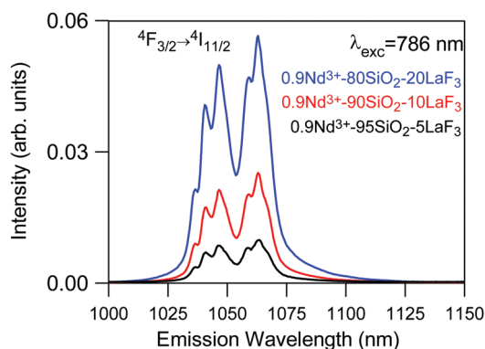
Fig. 10 Emission spectrum of 450^\circ\text{C} -6 h 0.9\text{Nd}^{3+}-\text{SiO}_2-\text{LaF}_3 GCs with three different crystalline fractions 5% (black), 10% (red) and 20% (blue) obtained under 786 nm excitation.
