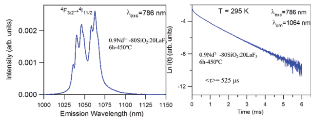
Fig. 9 Emission spectrum of 450^\circ\text{C} -6 h 0.9\text{Nd}^{3+}-80\text{SiO}_2-20\text{LaF}_3 sol and its corresponding semi-logarithmic plot of the experimental decay under excitation at 786 nm collecting the luminescence at 1064 nm.
