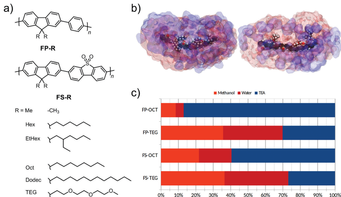
Fig. 1 (a) Structure of the fluorene co-phenyl ( FP-R ) and fluorene-co-dibenzo[b,d]thiophene sulfone ( FS-R ) polymer series where R is the alkyl group which is modified as shown; (b) molecular dynamics simulations of FS-Oct and FS-TEG in 1:1:1 water/methanol/TEA. TEA is shown in blue, and the water/methanol phase is shown in pink. In these simulations, FS-TEG draws a substantially higher concentration of water close to the polymer backbone at the expense of TEA; (c) bar chart showing fraction of volume within a 2 nm radius of the oligomer that is occupied by each component in the liquid medium: methanol (orange), water (red) and TEA (blue).
