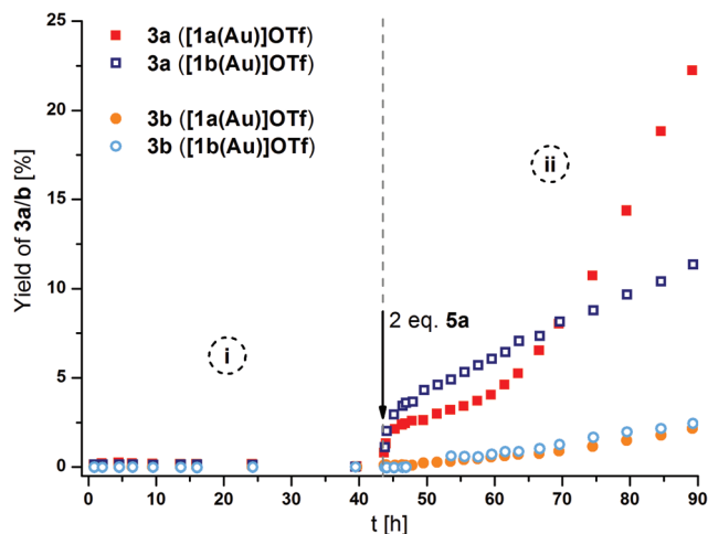
Fig. 10 Reaction profiles for ring-closing isomerisation of 2 to 3a (squares) by [\text{1a}(\text{Au})]\text{OTf} (solid symbols) and [\text{1b}(\text{Au})]\text{OTf} (hollow symbols), also showing the formation of the aromatic follow-up product 3b (circles) before (i) and after (ii) oxidation with 2 eq. 5a (with respect to catalyst; 3 mol% Au, [\text{2}]_0 = 60 \text{ mmol L}^{-1} , \text{CD}_2\text{Cl}_2 , 25 °C). For corresponding ^1\text{H} NMR spectra and TOF regression plots, s. Fig. S73, S75, and S76†
