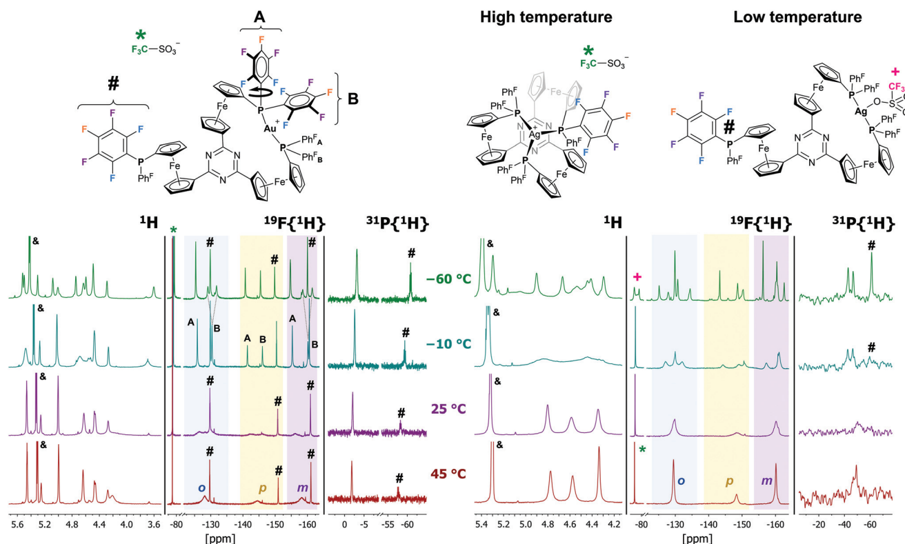
Fig. 5 Sections of the variable-temperature 1 H, 19 F{ 1 H}, and 31 P{ 1 H} NMR spectra of [1a F (Au)]OTf (left) and [1a F (Ag)]OTf (right) in CD 2 Cl 2 (δ: CHDCl 2 /CH 2 Cl 2 resonance; *: triflate anion resonance; +: split triflate anion resonance of [1a F (Ag)]OTf ; #: pendant P(Ph F ) 2 group). The shaded areas in the 19 F{ 1 H} NMR spectra correspond to the spectral regions of the ortho (blue), para (orange), and meta fluorine substituents of the P(Ph F ) 2 groups.
