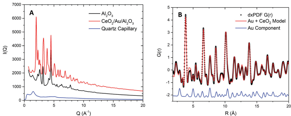
Fig. 2 Experimental DXP patterns, alumina subtraction and Fourier Transformation recorded at room temperature. (A) Integrated total scattering pattern relating to: a ceria alumina support Au inverse catalyst sample, a gamma alumina support and fused quartz capillary sample environment; illustrating the process for correction to arrive at the differential xPDF containing the fluorite ceria and metallic Au components. (B) Example fit to the initial differential xPDF G(r) for a biphasic model containing fluorite ceria and metallic Au components over a fitting region of 1.8 to 20 Å. The metallic Au component contribution is highlighted below the data to illustrate the presence of the metallic Au phase within the extracted differential xPDF G(r) . Typical fit residual, r_w = 0.1 .
