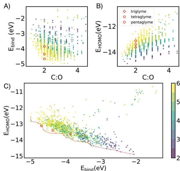
Fig. 3 The chemical space of Li-ether binding mapped by the number of ether groups: O: ion (color bar) and carbon and oxygen ratio (C:O) with G3, G4 and G5 marked by red square, pentagon and hexagon respectively. (A) E_{\text{bind}} of the Li-ether complexes. Weakly-binding outliers correspond ethers whose alkyl substituents crowd out oxygen-ion contact. (B) HOMO level of Li-ether complexes. (C) Scatter plots HOMO and E_{\text{bind}} overlaid with the Pareto front.
