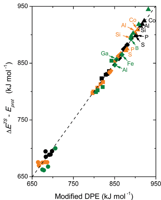
Fig. 9 Difference between DFT-derived (PW91) TS energies and gas-phase protonation energies ( \Delta E_{\text{int}}^{\text{TS}} - E_{\text{prot}} , Scheme 1) for H + shuttling (circles), CH 3 OH dehydration (squares), C 3 H 6 methyl-shift (diamonds) and C 6 H 10 ring-contraction (triangles) on Mo (orange) and W (black) POM and MFI (green), as a function of the modified DPE reflecting the sum of DPE and its compensation via ion-pair interactions. 33 Reproduced with permission from American Chemical Society.
