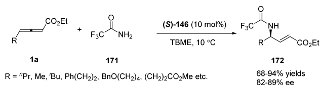
Scheme 53 Phosphine-catalysed \gamma -addition of trifluoromethyl-amide to \gamma -substituted allenolates.
