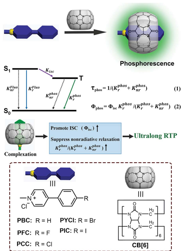
Scheme 1 Schematic illustration of the solid-state supramolecular strategy and Jablonski diagram for radiative and non-radiative processes. ( K_{nr}^{Fluo} is the radiative rate constant of the lowest excited singlet state S_1 ; K_{nr}^{Fluo} is the nonradiative rate constant of the lowest excited singlet state S_1 ; K_{isc} is the intersystem crossing rate constant from the excited singlet state to the triplet state; K_r^{Phos} is the radiative rate constant of the lowest excited triplet state T_1 ; K_{nr}^{Phos} is the nonradiative rate constant of the lowest excited triplet state T_1 ; \tau_{phos} is the lifetime of the excited triplet state; \Phi_{phos} is the quantum yield of phosphorescence; and \Phi_{isc} is the quantum yield of intersystem crossing from the excited singlet state to the triplet state; inset: the molecular structures of the guests and host).
