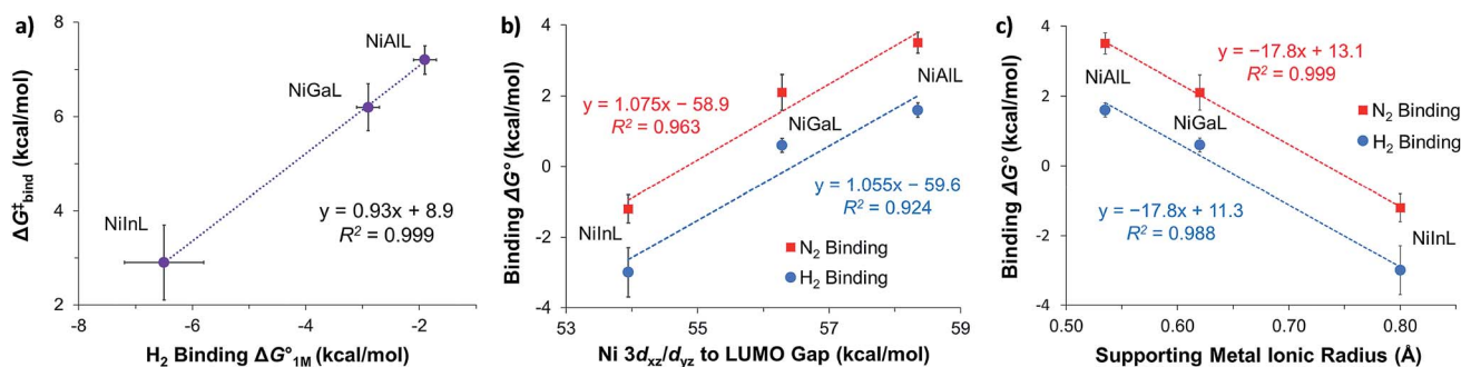
Fig. 7 (a) Plot of free energy barrier for H 2 binding ( \Delta G^\ddagger_{\text{bind}} ) vs. thermodynamic free energy for H 2 binding ( \Delta G^\circ_{1M} ), with the standard deviation in all values shown by error bars and all standard states defined to be [H 2 ] = 1 M in toluene- d 8 . (b–c) Plots of \Delta G^\circ for H 2 (blue circles) and N 2 binding (red squares) vs. Ni 3d xz /d yz to LUMO energy gap (b) and vs. supporting metal Shannon ionic radii (c). Ni 3d xz /d yz to LUMO energy gaps were measured experimentally by UV-Vis spectroscopy with transition assignments from TD-DFT calculations (see ESI† and Table 5).
