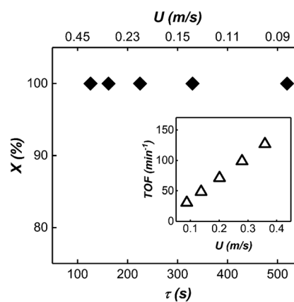
Fig. 10 1-Hexene conversion ( X ) versus bubble residence time ( \tau ) in scaled-up mesoreactor. Inset shows the turnover frequency of the reactor at different flow velocities. Turnover frequency is defined as number of moles of 1-hexene converted to product per number of moles of catalyst per unit time.
