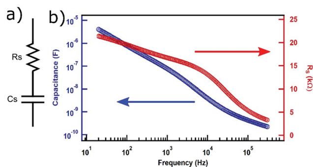
Fig. 4 (a) Equivalent circuit used for extracting capacitance ( C ) and equivalent series resistance ( R_s ) values from LCR meter. (b) Capacitance (blue) and equivalent series resistance (red) values as function of frequency.
