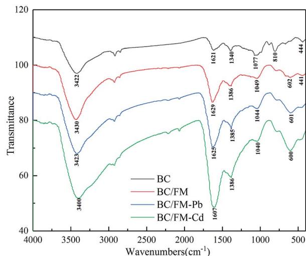
Fig. 9 FTIR spectra of BC, BC/FM, BC/FM-Pb, and BC/FM-Cd.
