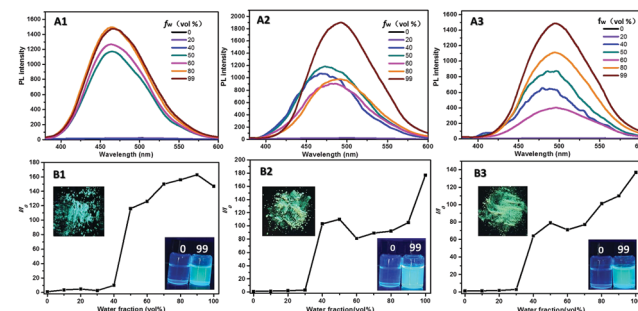
Fig. 3 Fluorescent spectra of TPE-L-Glu, cis -TPE-L-DGlu and trans -TPE-L-DGlu in THF/water mixed solvents with different f_w (A1–A3); plot of I_{00}/I_0 values versus f_w (B1–B3), where I_0 represents the emission intensity in THF. Concentration: 1 \times 10^{-5} M; excitation wavelength: 340 nm. Inset: Photographs of TPE-L-Glu, cis -TPE-L-DGlu and trans -TPE-L-DGlu in solid and THF/water mixtures with 0 and 99% f_w under 365 nm UV lamp.
