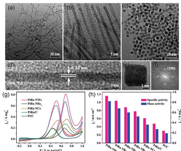
Fig. 15 TEM images of (a) PtRu NWs, (b) PtRu NRs, and (c) PtRu NCs. HRTEM images of an individual (d) PtRu NW and (e) PtRu NC, and the corresponding FFT pattern (f) of (e). (g) Electrocatalytic performances of PtRu nanocrystals and commercial Pt/C catalysts. CVs of (g) PtRu NWs, PtRu NRs, PtRu NCs, commercial PtRu/C, and commercial Pt/C for MOR in 0.1 M HClO 4 + 0.5 M CH 3 OH solution at a sweep rate of 50 mV s -1 . (h) Histograms of the mass and specific activities of different catalysts. Adapted with permission from ref. 187. Copyright 2017, American Chemical Society.
