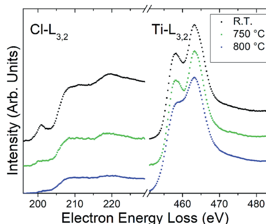
Fig. 4 Electron energy loss spectroscopy from a thin edge of a \text{Ti}_3\text{C}_2\text{Cl}_2 multilayer particle, showing the background subtracted and multiple scattering deconvolved Cl- and Ti-L 3,2 edges under ambient conditions and after heating at 750 and 800^\circ\text{C} . The spectra are normalized against the Ti-L 2 peak maximum and vertically separated for clarity.
