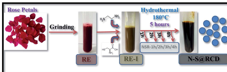
Scheme 1 Schematic for synthesis of N-S@RCD and intermediates.
