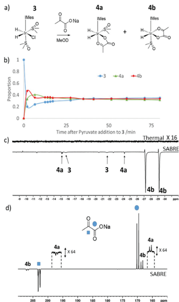
Fig. 3 (a) Reaction of 3 and pyruvate to form 4 (b) monitoring pyruvate addition to 3 using ^1\text{H} NMR spectroscopy. Pyruvate addition was made at room temperature to a solution of preformed 3 at 245 K before it was introduced into the spectrometer whose probe was at 245 K. There is therefore a rapid temperature change at the start of this data series. Upon shaking a solution of 3 and 4 with 3-bar p\text{-H}_2 for 10 seconds at (c) 65 G or (d) in a mu metal shield strongly hyperpolarised ^1\text{H} (c) or ^{13}\text{C} (d) resonances of 4b are observed compared to the thermal trace.
