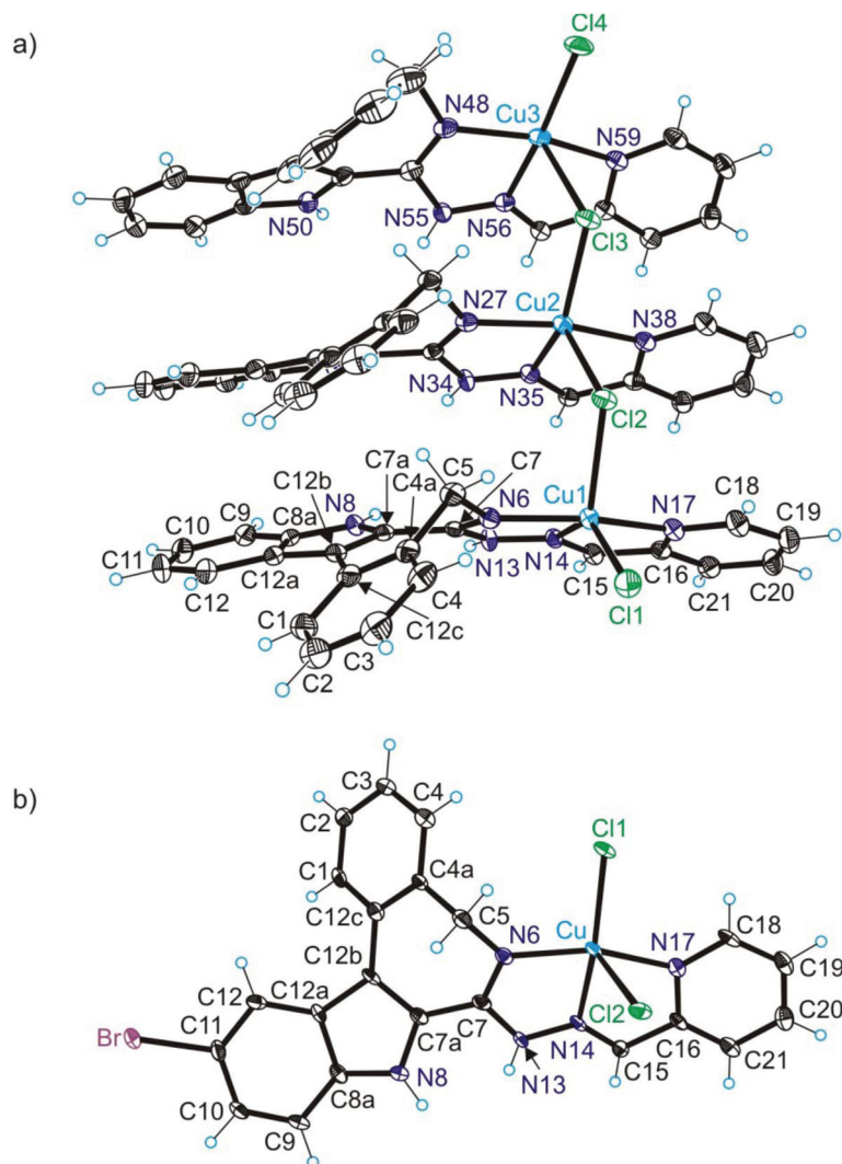
Fig. 1 ORTEP views of (a) the complex cation [Cu 3 Cl 4 (HL 1 ) 3 ] 2+ in 1 trim and (b) of [CuCl 2 (HL 2 )] in 2 . Selected bond distances (Å) and bond angles (deg) in 1 trim : Cu1–N6 1.994(2), Cu1–N14 1.991(2), Cu1–N17 2.044(2), Cu1–Cl1 2.2685(8), Cu1–Cl2 2.4382(7), N6–Cu1–N14 78.75(10), N14–Cu1–N17 77.92(9), Cu2–N27 1.990(2), Cu2–N35 1.975(2), Cu2–N38 2.034(2), Cu2–Cl2 2.4492(8), Cu2–Cl3 2.2781(8), N27–Cu2–N35 79.39(10), N35–Cu2–N38 78.63(10), Cu3–N48 1.995(3), Cu3–N56 1.959(2), Cu3–N59 2.044(2), Cu3–Cl3 2.6404(8), Cu3–Cl4 2.2116(8), N48–Cu3–N56 79.51(10), N56–Cu3–N59 79.20(10). Details of coordination geometry in 1 trim : τ 5 (Cu1) = 0.35, τ 5 (Cu2) = 0.25, τ 5 (Cu3) = 0.17; in 2 : Cu–N6 1.982(5), Cu–N14 1.971(5), Cu–N17 2.051(5), Cu–Cl1 2.2252(16), Cu–Cl2 2.5762(17), N6–Cu–N14 79.7(2), N14–Cu–N17 78.8(2). Details of coordination geometry in 2 : τ 5 (Cu) = 0.06.
