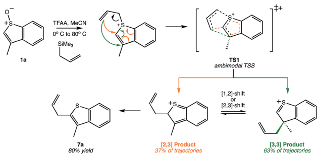
Scheme 3 A recently published synthetic example of a similar reaction that may involve a PTSB. 25,26 This example corresponds to reactant 1a in this scheme of the original publication.
