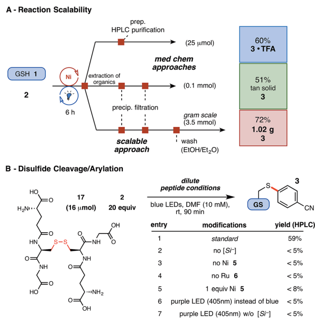
Fig. 4 (A) Demonstration of reaction scalability for the Ni/photoredox thioarylation of peptides (see ESI† for details); isolated yields reported. (B) Dilute conditions employed: 5 mol% Ni 5, 2 mol% Ru 6, and 1.5 equiv. silicate 4. HPLC yields reported via product/internal standard ratios.
