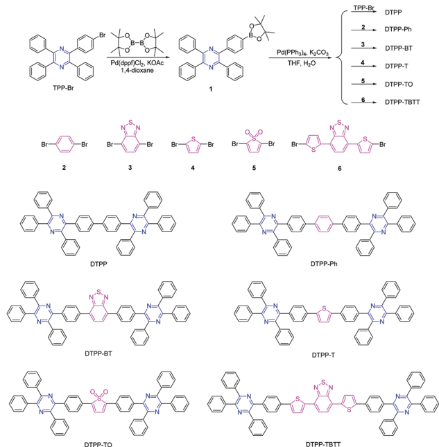
Scheme 1 Synthetic routes to TPP derivatives of DTPP, DTPP-Ph, DTPP-BT, DTPP-T, DTPP-TO and DTPP-TBTT.
