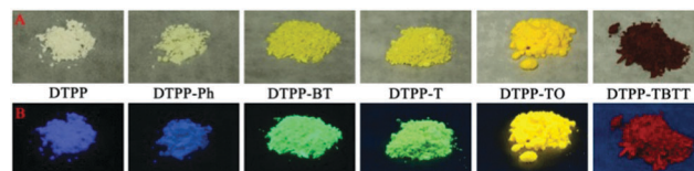
Fig. 1 Photos of DTPP, DTPP-Ph, DTPP-BT, DTPP-T, DTPP-TO and DTPP-TBTT in amorphous powders, taken under the illumination of (A) a daylight lamp and (B) a UV lamp (365 nm).
