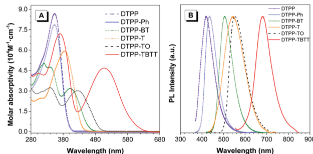
Fig. 2 (A) Absorption of THF solutions (10 μM) and (B) photoluminescence spectra of films of DTPP, DTPP-Ph, DTPP-BT, DTPP-T, DTPP-TO and DTPP-TBTT.
