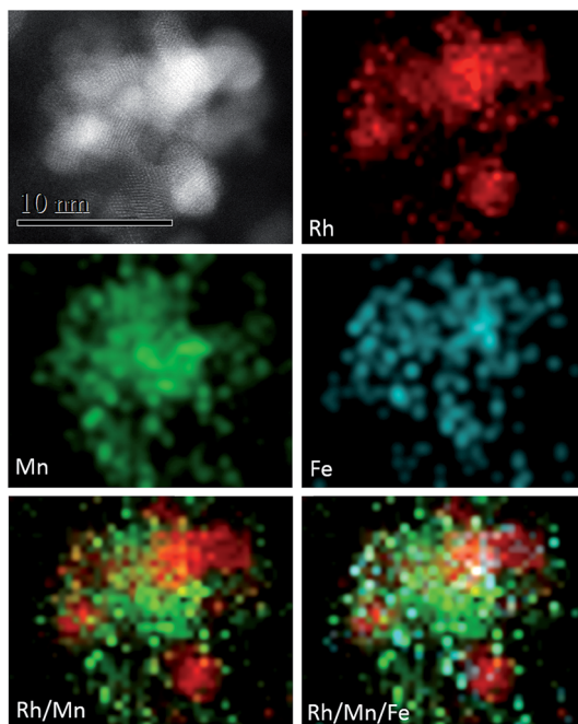
Fig. 4 HAADF-STEM image and corresponding EDX elemental mapping of Fe, Mn and Rh, and a superimposed elemental map of the reduced Rh–Mn–Fe/SiO 2 catalyst showing an intimate contact of the three elements.
