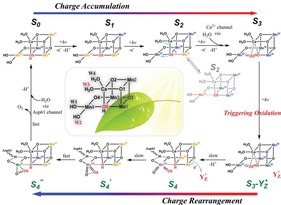
Fig. 2 Proposed catalytic mechanism for water oxidation by Mn_4CaO_5 cluster in PSII involving Mn^{VII} -dioxo species. Charge disproportionation of Mn_4CaO_5 cluster at the S_3 - Y_Z' state after accumulation of three charges, i.e. , charge rearrangement, leads to the formation of a super-active S_4' [III, III, IV, VII] state after the S_3 \rightarrow S_4 step. An O–O bond forms within the Mn^{VII} -dioxo site (between W2 and O5) during the S_4 \rightarrow S_4' step. W2, O5, and W3 all participate in O_2 evolution.
