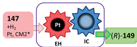
Scheme 44 Cascade enantioselective hydrogenation (EH) and intramolecular cyclization (IC) of 2-oxoglutaric acid using Pt catalyst modified by cinchona alkaloid CM2*. 196
