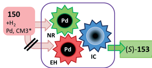
Scheme 45 Cascade nitro group reduction (NR), EH and IC over cinchonidine modified Pd catalyst. 202
