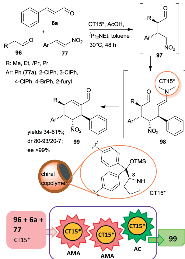
Scheme 29 Tricomponent asymmetric triple cascade reaction catalysed by multi-hollow copolymer microparticles containing immobilized CA6*; AC: aldol condensation. 163
