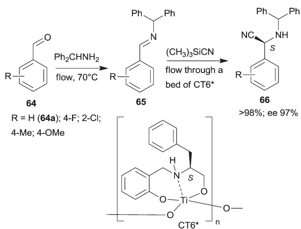
Scheme 20 Sequential imine formation and asymmetric cyanation catalysed by self-supported chiral titanium cluster CT6*. 139
