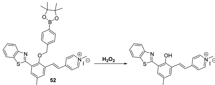
Scheme 48 A NIR-mitochondria targeting ESPT fluorescent probe 52 that allows for the ratiometric detection of hydrogen peroxide in A549 cells. Measurement conditions: HEPES/ACN (50 : 50) pH = 7.4.
