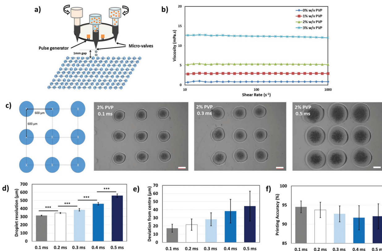
Fig. 3 (a) Schematic drawing of drop-on-demand microvalve-based printing for PVP-based bio-inks. (b) Rheological characterization of different PVP-based bio-inks (0–3% w/v) from 10–1000 s^{-1} . (c) Arrays of 3 × 3 PVP droplets are printed at a constant spacing of 600 \mu m (centre marked by white x) and representative images of the printed PVP droplets at different valve opening times (VOTs) from 0.1–0.5 ms; scale bar: 200 \mu m . ImageJ analysis of the (d) droplet resolution, (e) deviation from the centre and (f) printing accuracy.
