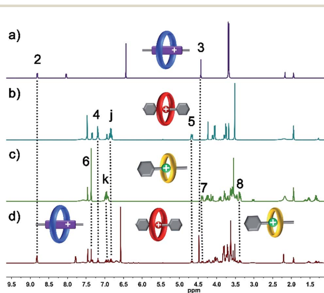
Fig. 1 Partial 1 H NMR spectra (400 MHz, 298 K, \text{CD}_3\text{CN} ) of (a) 1 : 1 mixture of BPP34C10 \supset BPY 2+ , (b) 1 : 1 mixture of DB24C8 \supset DBA, (c) 1 : 1 mixture of B21C7 \supset BAA and (d) equal molar mixture of BPP34C10, DB24C8, B21C7, BPY 2+ , DBA and BAA.
