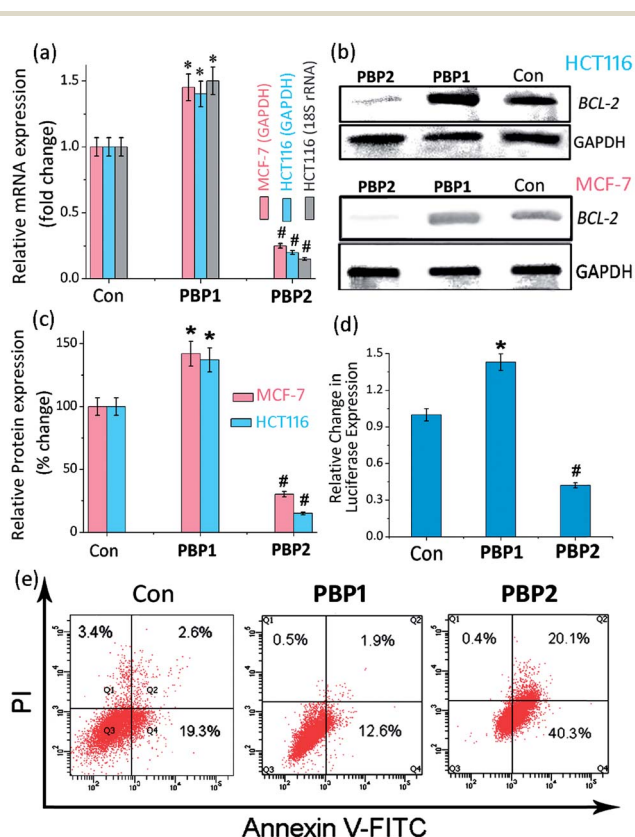
Fig. 4 (a) Determination of the transcriptional regulation of BCL-2 mRNA in the presence of IC 50 doses (24 h) of PBP1 or PBP2 in cancer cells (MCF-7 and HCT116) via qRT-PCR and quantified by double delta C t analysis using GAPDH and 18S rRNA as reference genes. Data is presented in terms of fold change (the expression of control is 1 fold). The data are shown as mean ± SD. * P < 0.05, # P < 0.01, versus untreated cancer cells. (b) Immunoreactive bands of the BCL-2 protein were analyzed via western blot in MCF-7 and HCT116 cells. The data are shown as mean ± SD. * P < 0.05, # P < 0.01, versus untreated cancer cells. (c) The protein expression of the BCL-2 protein in the presence of IC 50 doses (24 h) of PBP1 or PBP2 in MCF-7 and HCT116 cancer cells. (d) The relative luciferase expression in the LB322 BCL-2 promoter containing firefly plasmid normalized with pRL-TK Renilla plasmid (FF/RL) upon treatment with 5 μM of PBP1 and PBP2 in HCT116 cells, data shown here as mean ± SD. * P < 0.05, # P < 0.01, versus untreated cancer cells. (e) Flow cytometric analysis upon treatment with 5 μM of PBP1 and PBP2 in serum starved MCF-7 cells, Q3, Q4, Q2, and Q1 indicate healthy cells, early, late apoptotic, and necrotic cells, respectively.
