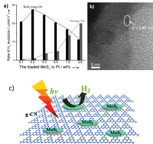
Fig. 6 (a) The rate of H 2 production over mpc-C 3 N 4 loaded with different amounts of MoS 2 or Pt, (b) TEM image of MoS 2 /g-C 3 N 4 and (c) illustration of the deposition of layered MoS 2 on the surface of g-C 3 N 4 for photocatalytic H 2 evolution. Reprinted with permission from ref. 57. Copyright 2013, Wiley-CVH.
