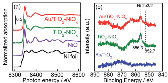
Fig. 4 (a) Ni K-edge XANES spectra of Ni foil, NiO, \text{TiO}_2\text{-NiO}_x(0.5) and \text{Au}(1.0)/\text{TiO}_2\text{-NiO}_x(0.5) ; (b) XPS spectra of \text{Au}(1.0)/\text{TiO}_2\text{-NiO}_x(0.5) and \text{TiO}_2\text{-NiO}_x(0.5) around Ni 2p components.
