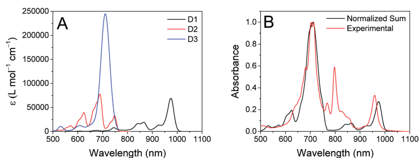
Fig. 8 Left: Calculated vibronic transitions from the ground state to the D1 (black), D2 (red) and D3 (blue) states of \text{PDI}^- . Right: Sum of the three calculated vibronic spectra (black) compared to the experimentally determined spectrum of \text{PDI}^- , normalized to the maximum value.
