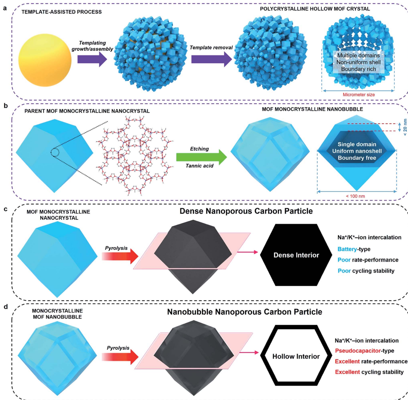
Fig. 1 (a) Schematic illustration of the synthesis of hollow MOF crystals via traditional templating methods. (b) Schematic illustration of the spatially controlled etching to produce monocryalline MOF nanobubbles. The nanobubbles are less than 100 nm in size, and have a monocryalline shell with a thickness less than 20 nm. (c) Schematic illustration of the pyrolysis of MOF nanocrystals and description of Na + /K + ion intercalation performance of the carbonized ZIF-8 nanocrystals (denoted as 'non-hollow carbon nanoparticles'). (d) Schematic illustration of the pyrolysis of MOF nanobubbles and description of Na + /K + ion intercalation performance of the carbonized MOF nanobubbles (denoted as 'hollow carbon nanobubbles').
