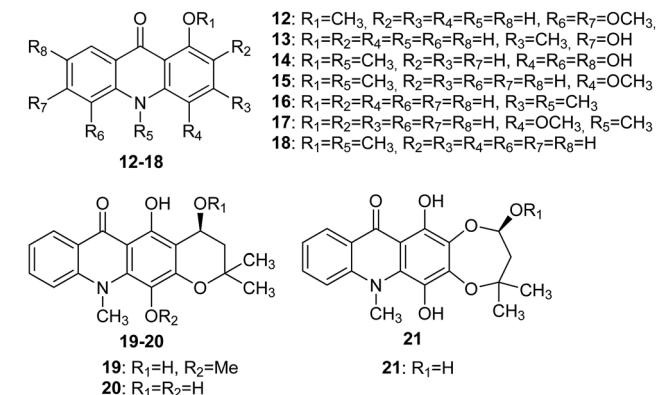
Fig. 4 Structures of acridones (12–21). 36
