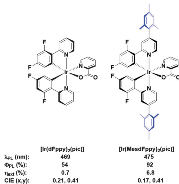
Fig. 2 FIrpic and its mesityl functionalised analogue. The mesityl functionality confers improved properties in virtually all important metrics, including solution state \Phi_{\text{PL}} , as well as \eta_{\text{ext}} values and CIE coordinates for comparable solution processed device architectures. This comes only at the expense of a small red-shift in solution state \lambda_{\text{max}} .
